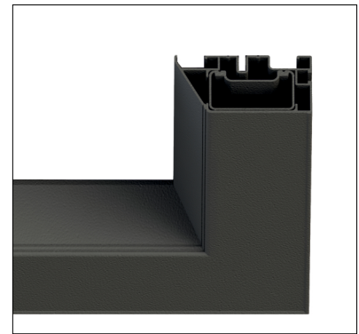
Special shape of aluminium frame with bevel of inner edge for higher viewing angle up to 30°
