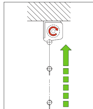
Slow return system for a slow and controlled rolling up of the screen surface
